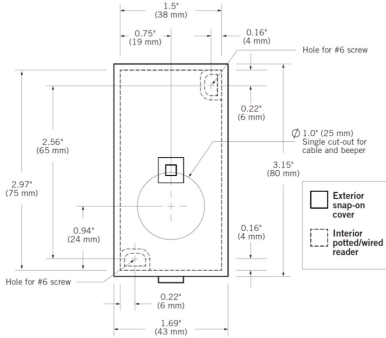
FRONT VIEW
