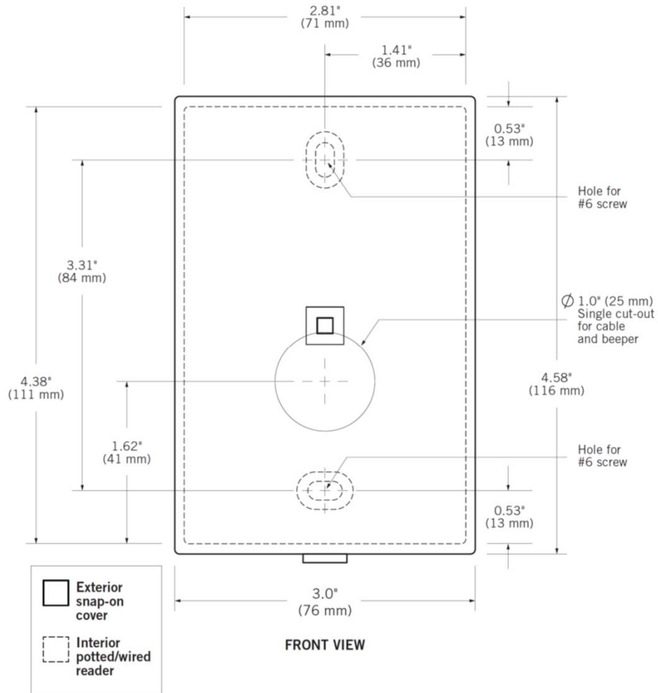
FRONT VIEW
