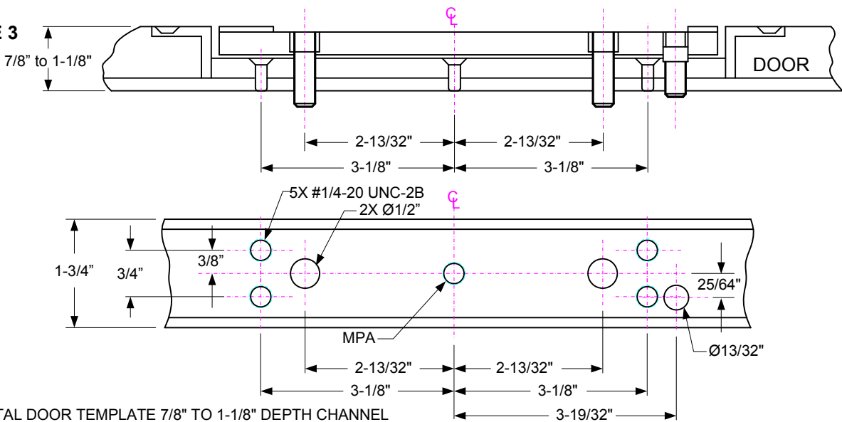
METAL DOOR TEMPLATE 7/8" TO 1-1/8" DEPTH CHANNEL
