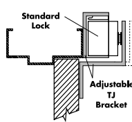
FIG. 1D Top Jamb Installation
