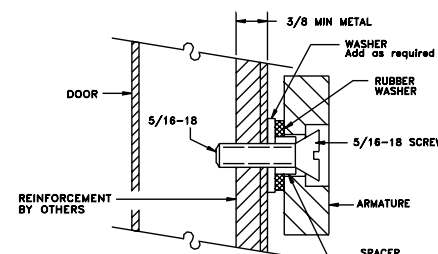
FIG. 2C REINFORCED DOOR
