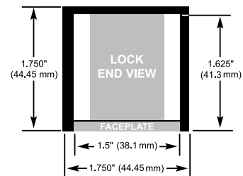
Figure 4: End View
