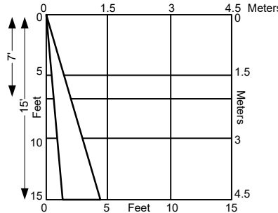
Side view of coverage range with -14° aim
