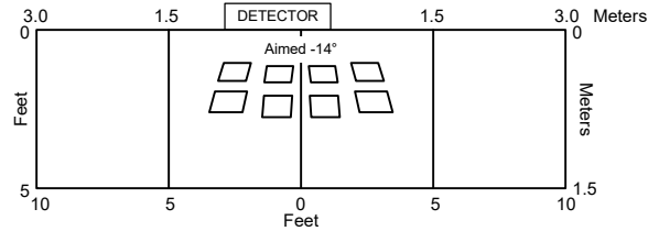
Top view of coverage pattern on the floor at 7' wall mount height with -14° aim
