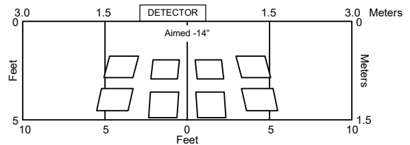
Top view of coverage pattern on the floor at 15' wall mount height with -14° aim
