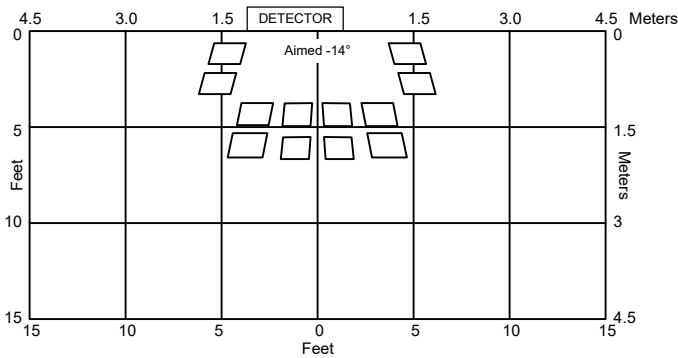
Top view of coverage pattern on the floor at 7' wall mount height with -14° aim
