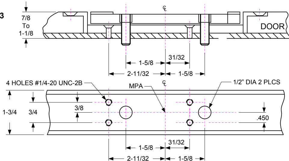
METAL DOOR TEMPLATE 7/8" TO 1-1/8" DEPTH CHANNEL
